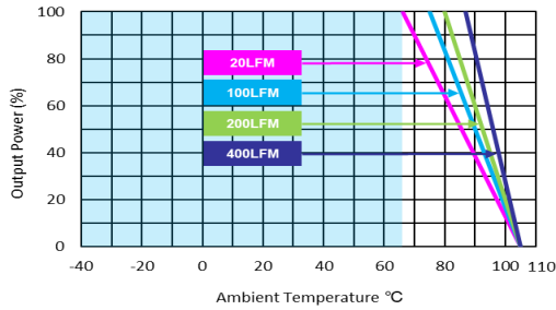
MKWI40-24S033, MKWI40-48S033 Derating Curve without Heatsink
