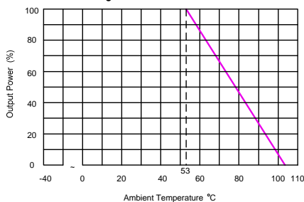
MJW25-24S033, MJW25-48S033 Derating Curve without Heatsink
