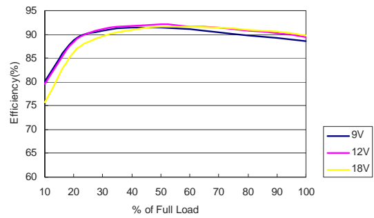
MKW50-12S05 Efficiency vs Load Current
