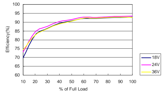
MKW50-24S05 Efficiency vs Load Current
