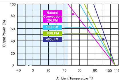
MKW50-12S12, MKW50-12S15 Derating Curve without Heatsink
