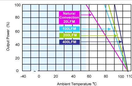
MKW50-12S12, MKW50-12S15 Derating Curve with Heatsink
