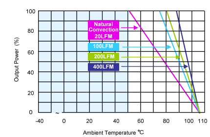
MKW50-12S05 Derating Curve with Heatsink
