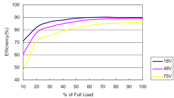
MKWI40-48S15 Efficiency vs Load Current
