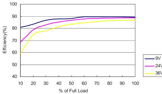
MKWI40-24S12 Efficiency vs Load Current
