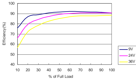
MKWI40-24S033 Efficiency vs Load Current
